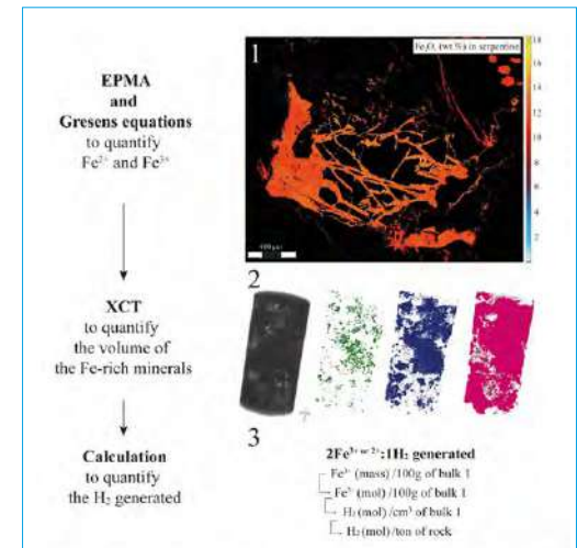
▲ Hydrogen quantification workflow with 1- the Fe^{3+} map for a mineral of interest (here the serpentine), 2- the volume determination for each mineral by performing XCT (green is oxide, blue is for mafic minerals, and pink is for the feldspathic matrix), and 3- the H_2 calculation applied for the whole rock.
